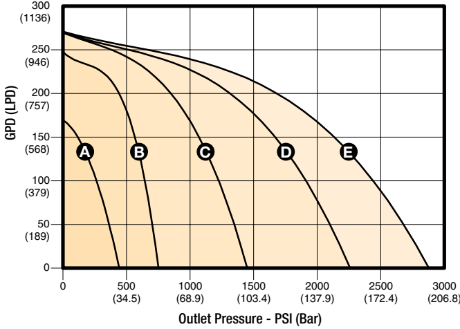
5/8" Plunger (PCI-450-63)
