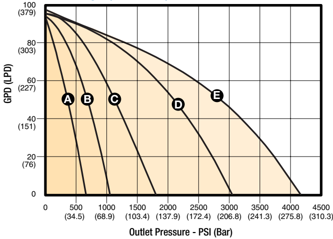
3/8" Plunger (PCI-250-38)
