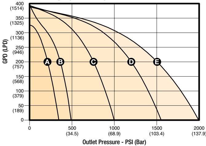
5/8" Plunger (PCI-450-63)
