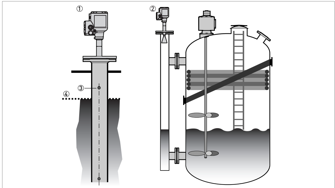
Figure 3-10: Installation recommendations for standpipes (stilling wells and bypass chambers)
