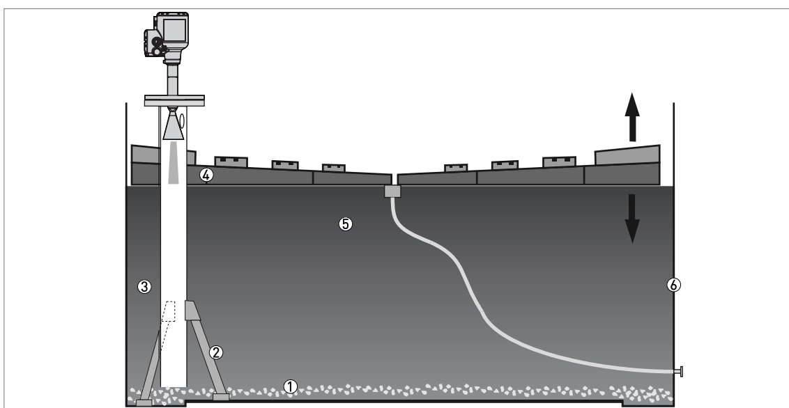
Figure 3-11: Floating roofs
